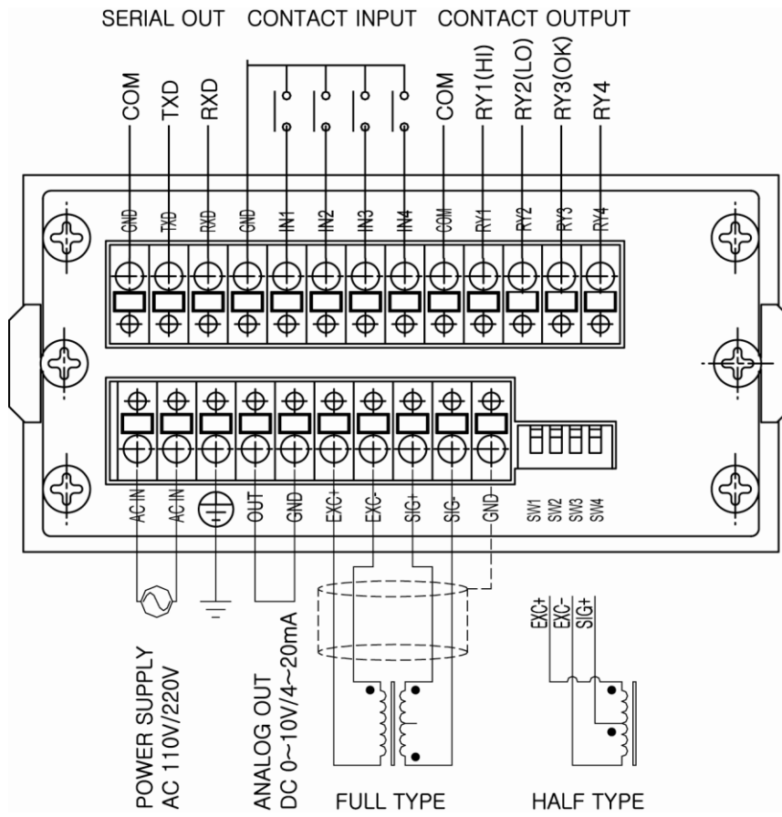
< Wiring Diagram >
